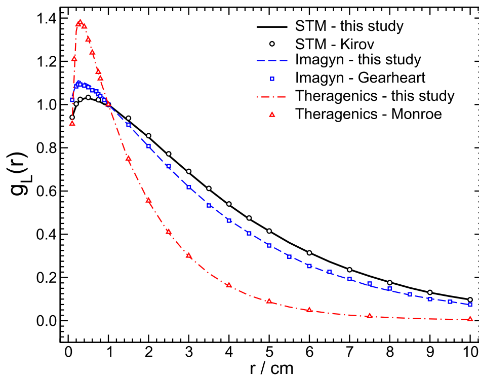
Figure 3.11: Radial dose function g_L(r) , for the three sources. Voxel sizes are: 0.1 \text{ mm}^3 for r \leq 1 \text{ cm} , 0.5 \text{ mm}^3 for 1 \text{ cm} < r \leq 5 \text{ cm} , 1.0 \text{ mm}^3 for 5 < r \leq 10 \text{ cm} . Lines are values calculated in this study and symbols are values calculated by other authors. 34, 37, 45
