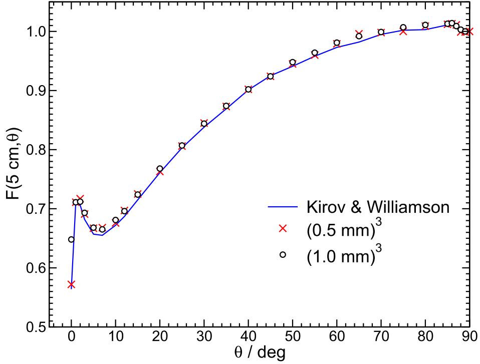
Figure 3.7: Anisotropy function at r = 5 cm for the STM1251 source. The plot shows the anisotropy factor calculated with voxels of (0.5 \text{ mm})^3 and (1.0 \text{ mm})^3 as well as values calculated by Kirov and Williamson et al. 34 using a point estimator. There is a significant voxel size effect at 0^\circ only.
