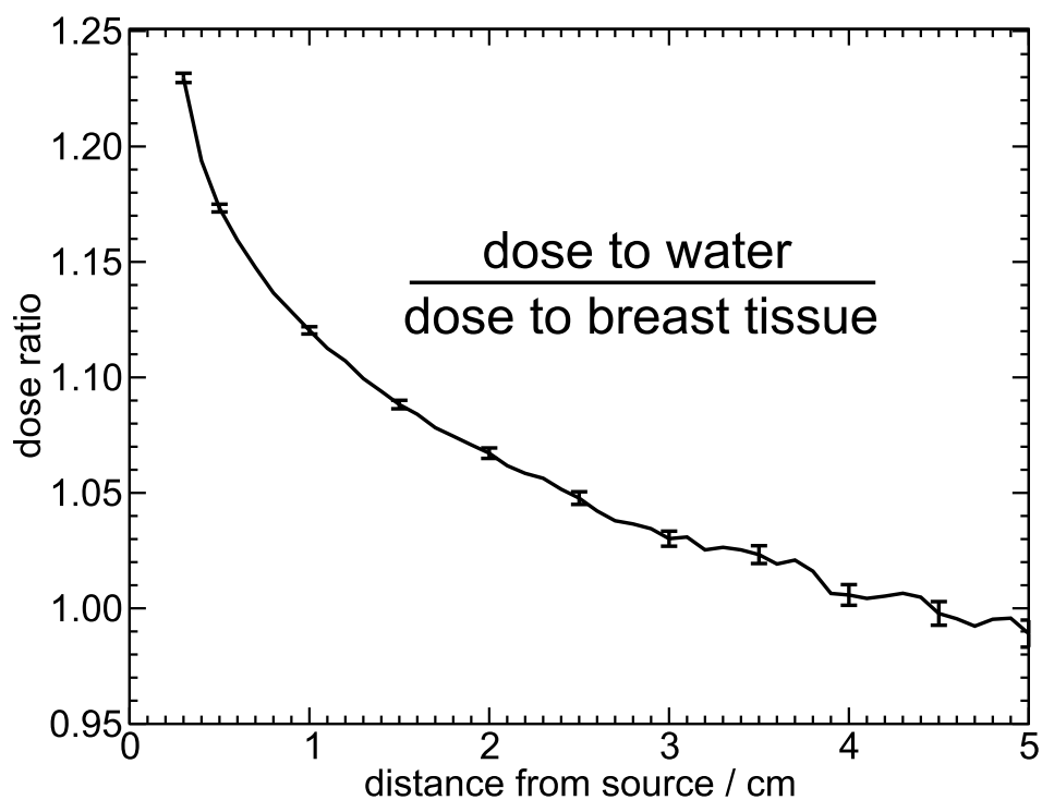
Figure 5.5: Ratio of dose calculated in water to dose calculated in breast tissue (see Table 5.1) for the Xofig source. The dose to water is \sim 23\% higher than the dose to tissue close to the source. The dose to water is less than the dose to breast tissues at distances greater than \sim 5 cm.
