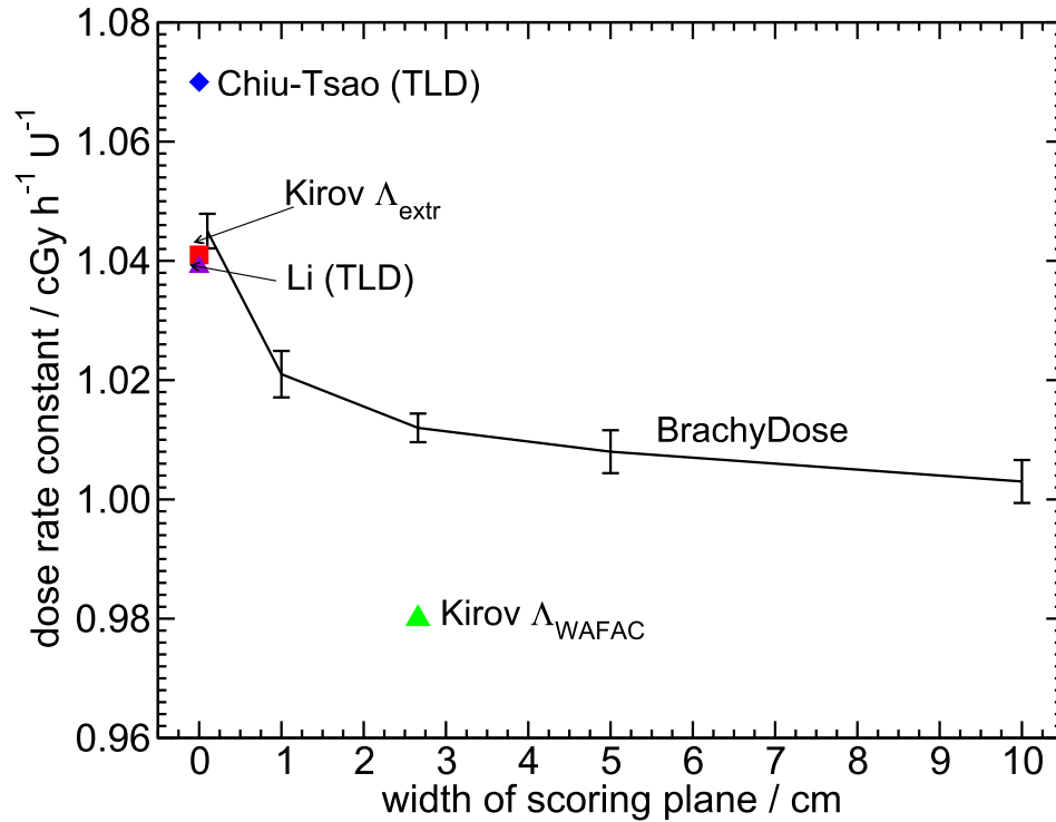
Figure 3.8: Variation of the dose rate constant for the STM1251 ^{125}\text{I} seed. Dose rate constants were determined using air kerma strengths averaged over voxels that were 0.5 mm thick and had varying widths. The face of the scoring voxels were located 10 cm from the source. For comparison, values of the dose rate constants calculated or measured by other authors 34–36 are also included. The WAFAC calculation by Kirov and Williamson is shown at a “width” of 2.7 cm. Kirov and Williamson’s point kerma extrapolated estimate and TLD measurements are shown at 0 cm. Uncertainties on Kirov’s calculations, Li’s 35 measurements and Chiu-Tsao’s 36 measurements are 2.5%, 7% and 5.5% respectively.
