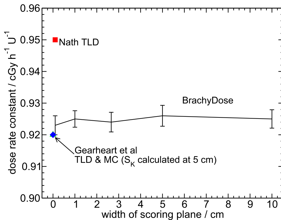
Figure 3.9: As in figure 3.8 for the Imagyn ^{125}\text{I} source. Ibbott et al 's 40 calculated value and TLD measurements 37–39 are shown at 0 cm. The uncertainty on the TLD measurement by Gearheart et al 37 and Nath 38 are 7.7% and 10% respectively.
