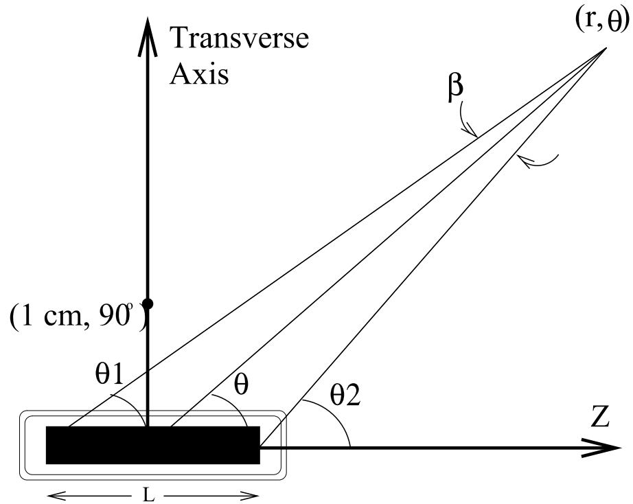
Figure 2.1: Geometry of the TG-43 dosimetry formalism. L is defined as the active length of the source and is related to the spatial extent of radioactive material within the source. \theta_1 and \theta_2 are the angles defined by the z axis and the lines running from z = \pm L/2 to the point of interest, (r, \theta) . \beta is the angle subtended by the active length, L , at the point of interest.
