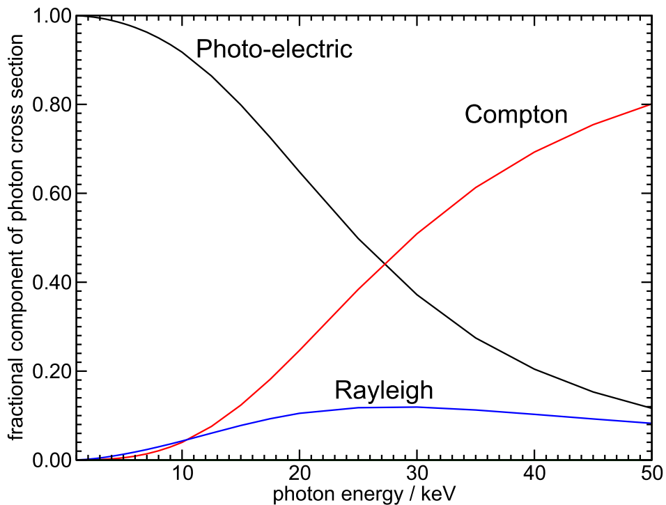
Figure 5.4: Relative fraction of Rayleigh, photo-electric and Compton scatter components of the total photon cross section of water.
