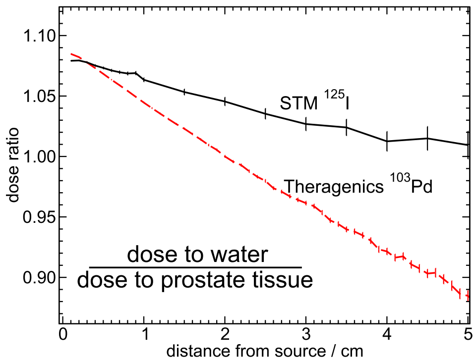
Figure 5.6: Ratio of dose calculated in water to dose calculated in prostate tissue for the Theragenics ^{103}\text{Pd} and STM ^{125}\text{I} sources. The dose to water significantly overestimates the dose to tissue near the source and then underestimates the dose as the distance from the source increases. The effect is more pronounced for the Theragenics source due to the lower average energy of ^{103}\text{Pd} .
