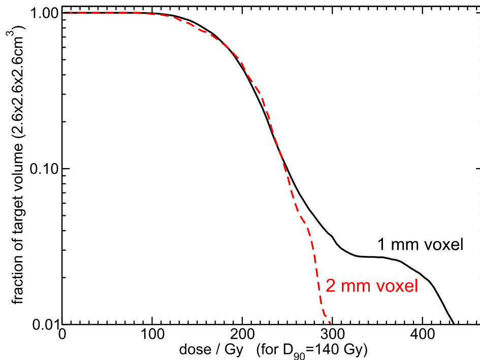
Figure 5.9: Effect of voxel size on dose-volume histograms. The dose volume histogram in this figure was calculated for 1 \times 1 \times 1 \text{ mm}^3 and 2 \times 2 \times 2 \text{ mm}^3 voxels in a 2.6 \times 2.6 \times 2.6 \text{ cm}^3 region. The region contains 125 ^{125}\text{I} seeds arranged in a 5 \times 5 \times 5 grid with a seed separation of 0.5 cm. All seeds were randomly shifted up to 0.5 mm in each direction to avoid artifacts in the DVH resulting from calculating dose in voxels (explained in text). Both DVH's are normalized to D_{90} = 140 \text{ Gy} in the 1 mm voxels.
