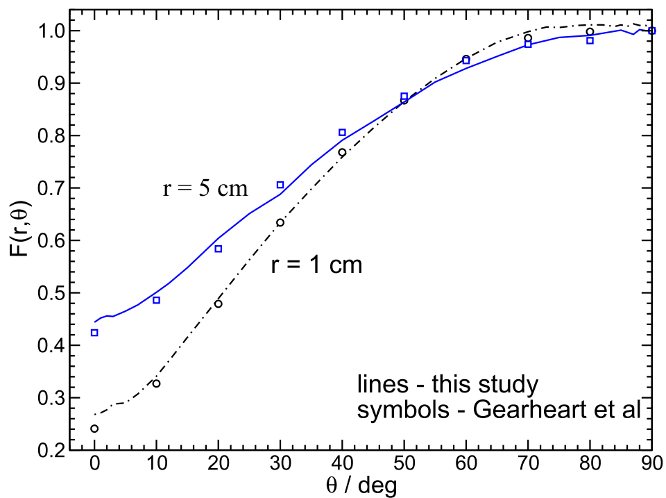
Figure 3.13: Comparisons of anisotropy data calculated for the Imagyn isoStar TM125 source with values calculated by Gearheart et al. 37 Voxel sizes are (0.1 \text{ mm})^3 at 1 cm and (0.5 \text{ mm})^3 at 5 cm.
