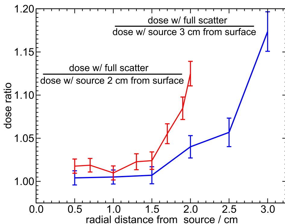
Figure 5.2: Ratio of dose with and without a full backscattering medium present for the Xofter Axxent source. When the source is located 3 cm from the surface of a phantom the full scatter calculation overestimates dose by 17% at the surface of the phantom. The same calculation with the source placed 2 cm from the surface results in an overestimate of 12% by the full scatter calculation.
