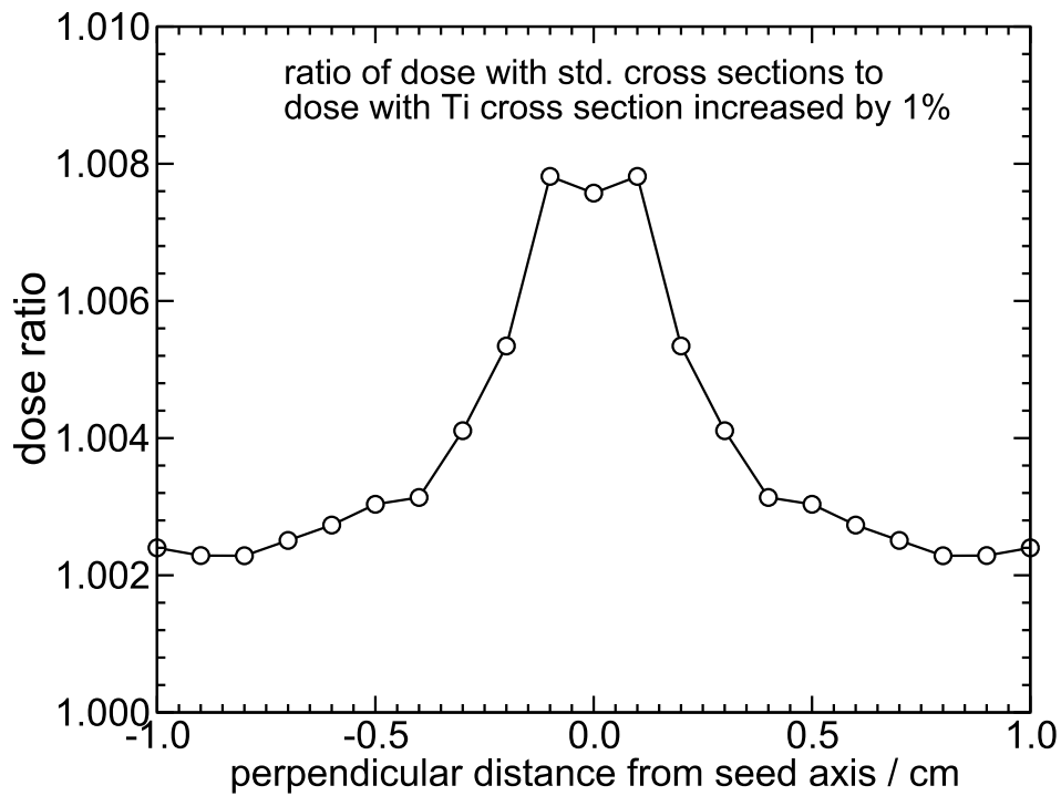
Figure 3.15: Ratio of the dose calculated using the standard cross sections to dose calculated with the cross section of the Ti encapsulation increased by 1%. The dose ratio profile shown was taken perpendicular to the seed axis and 0.5 cm from the source centre. A 1% increase in the cross section of Titanium leads to a decrease in dose of 0.8% at 0°.
