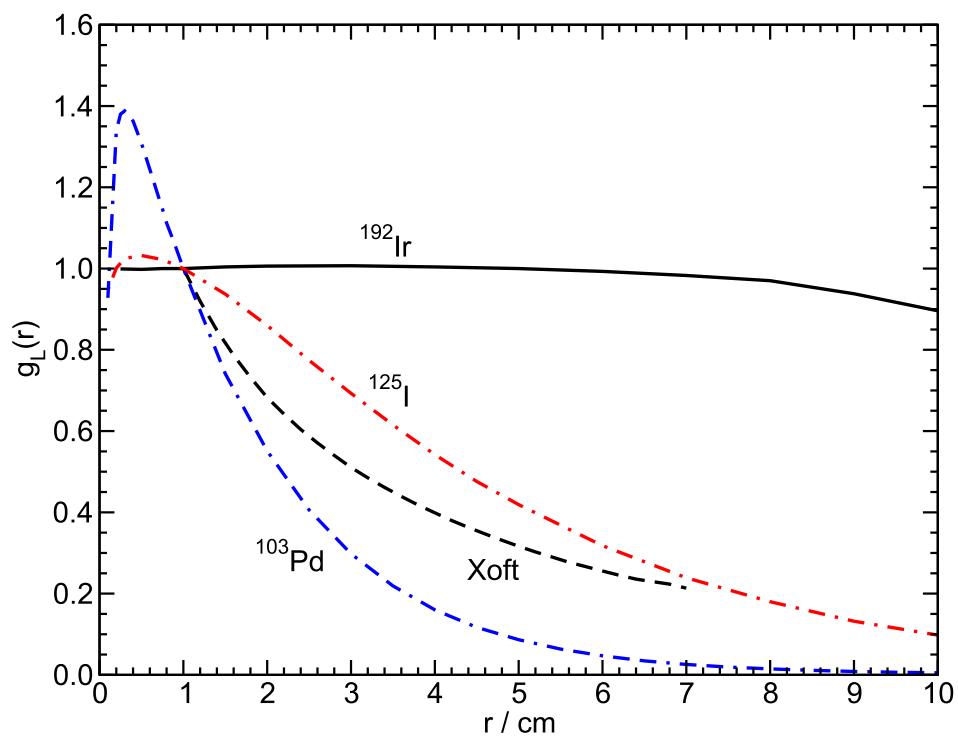
Figure 1.2: Comparison of radial dose functions, g_p(r) , of the Axxent source with ^{192}\text{Ir} , ^{125}\text{I} and ^{103}\text{Pd} sources. The Axxent source has a dose fall off similar to ^{125}\text{I} and ^{103}\text{Pd} sources while achieving a dose rate as high as an ^{192}\text{Ir} source.
