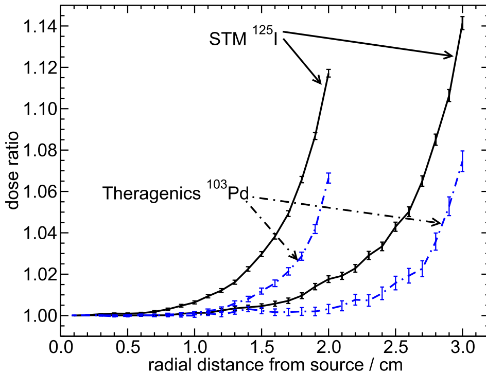
Figure 5.3: As in figure 5.2 but for the STM ^{125}\text{I} and Theragenics ^{103}\text{Pd} source. With the sources placed 3 cm from the surface of the phantom the full scatter calculation overestimates dose by approximately 14% and 8% for ^{125}\text{I} and ^{103}\text{Pd} , respectively.
