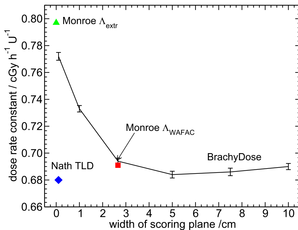
Figure 3.10: As in figure 3.8 for the Theragenics ^{103}\text{Pd} seed. The WAFAC calculations by Monroe and Williamson 45 are shown at a “width” of 2.6 cm. Monroe and Williamson’s point kerma extrapolated estimate and Nath et al ’s 43 TLD measurements are shown at 0 cm. Uncertainties on Monroe and Williamson’s MC results are 3%.
