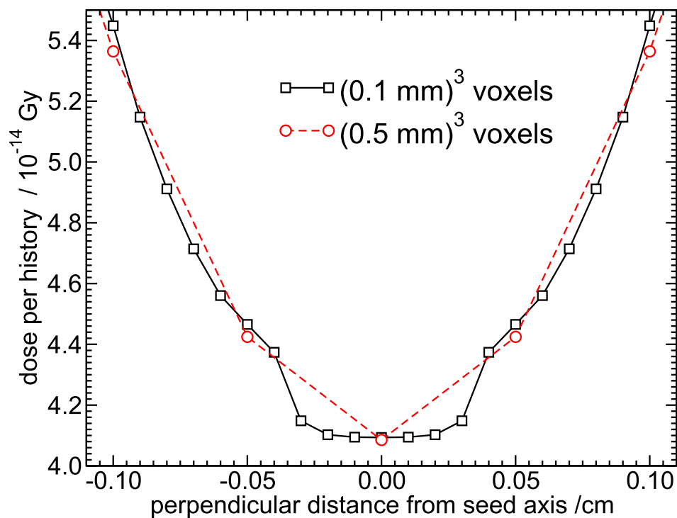
Figure 3.14: Dose profile perpendicular to source axis located 0.5 cm from the Imagyn source centre. Voxels are (0.1 \text{ mm})^3 and (0.5 \text{ mm})^3 . It is evident from this plot that decreasing the voxel size further would likely have no effect on the anisotropy function values calculated at \theta = 0^\circ .
