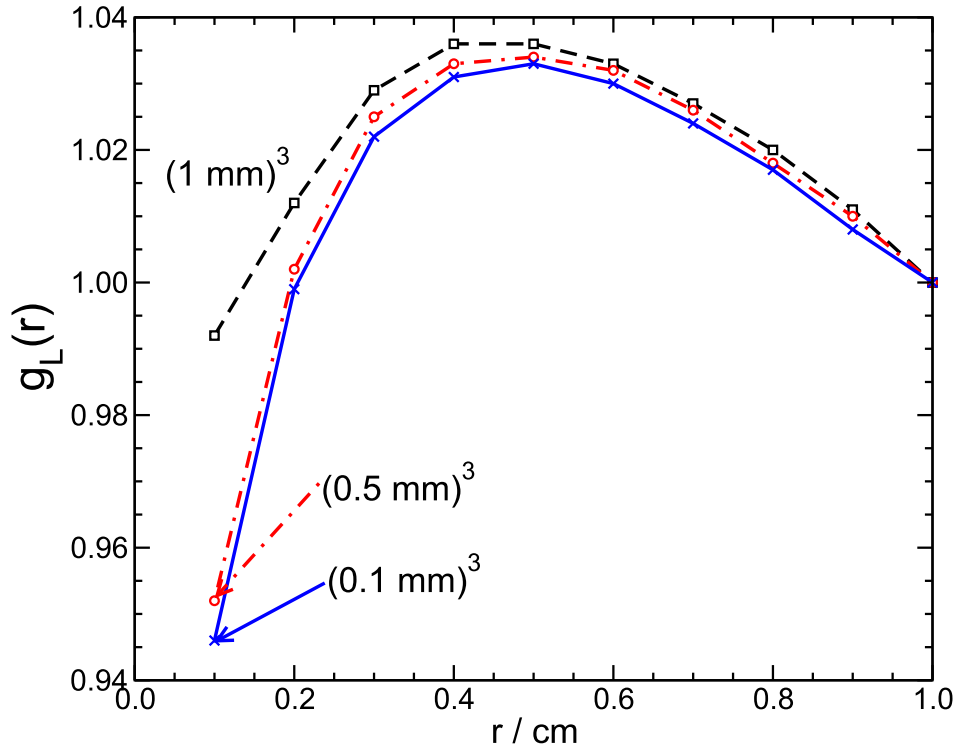
Figure 3.5: Calculated radial dose function, g_L(r) , for the STM1251 source. The plot shows the g_L(r) calculated with voxels of (0.1 \text{ mm})^3 , (0.5 \text{ mm})^3 and (1.0 \text{ mm})^3 . The radial dose function value calculated in a (1.0 \text{ mm})^3 voxels is 5% greater than the value calculated in a (0.1 \text{ mm})^3 voxel at 1 mm. The calculations for the (0.5 \text{ mm})^3 and (0.1 \text{ mm})^3 differ by less than 0.7% for distances less than 1 cm from the source.
