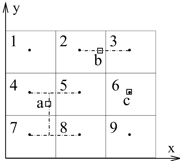
Figure 1.1: 2-dimensional example of the dose interpolation implemented in TG43extract. The method used for calculating dose at points a, b and c is given in the text.
