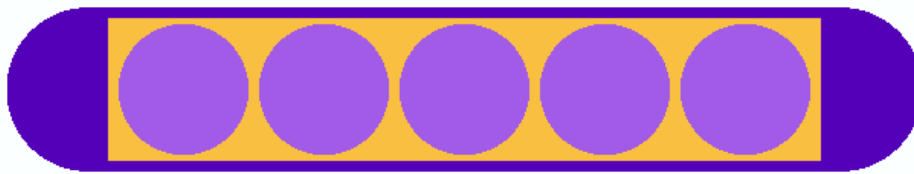
Figure 3.2: Cross section of the Imagyn isoStar TM ( ^{125}\text{I} ) seed. Drawing is to scale and a detailed description is given in the text.
