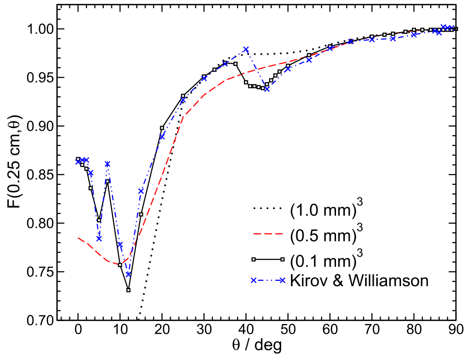
Figure 3.6: Anisotropy function at r = 0.25 cm for the STM1251 source. The plot shows the anisotropy factor calculated with voxels of (0.1 \text{ mm})^3 , (0.5 \text{ mm})^3 and (1.0 \text{ mm})^3 as well as values calculated by Kirov and Williamson 34 using a point estimator.
