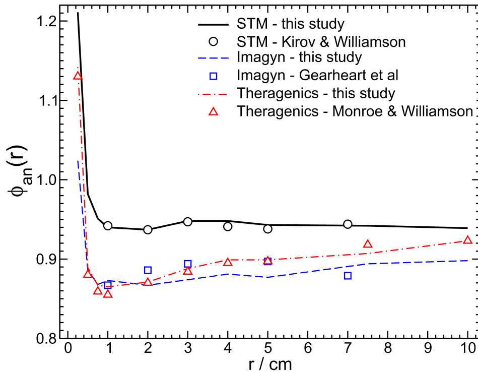
Figure 3.17: Comparisons of anisotropy factor, \phi_{an}(r) , data calculated in this study with the values calculated by other authors. 34,37,45 The 2% discrepancies seen for the Imagyn ^{125}\text{I} source are likely a result of the differences seen in the calculated anisotropy function, F(r,\theta) , of this study and Gearheart et al 's and the poor angular resolution used in their paper.
