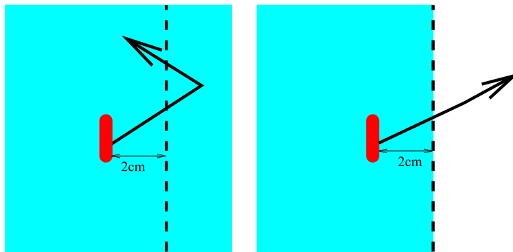
Figure 5.1: Calculation setup for comparing the ratio of dose with and without a full backscattering medium present. In this case the source is located 2 cm from the face of a phantom.
