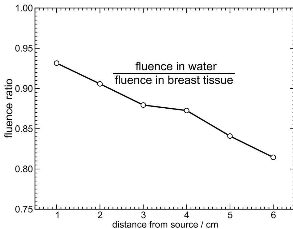
Figure 5.8: Ratio of photon fluence in water to fluence in breast tissue for the Xoft source at 50 kV calculated using FLURZnrc.
