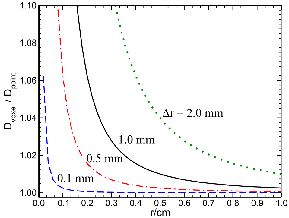
Figure 3.4: Ratio of the average dose in spherical shells of thickness \Delta r (calculated using eq. 3.4) to dose at the midpoint of the shell for a point source with a 1/r^2 distribution. Four different shell thicknesses are included. Scoring in shells of 1 mm thickness leads to dose overestimates of 2.8% and 0.25% at 3 mm and 10 mm respectively. Decreasing the thickness of the shell to 0.1 mm leads to overestimates of less than 0.1% at the same two points.
