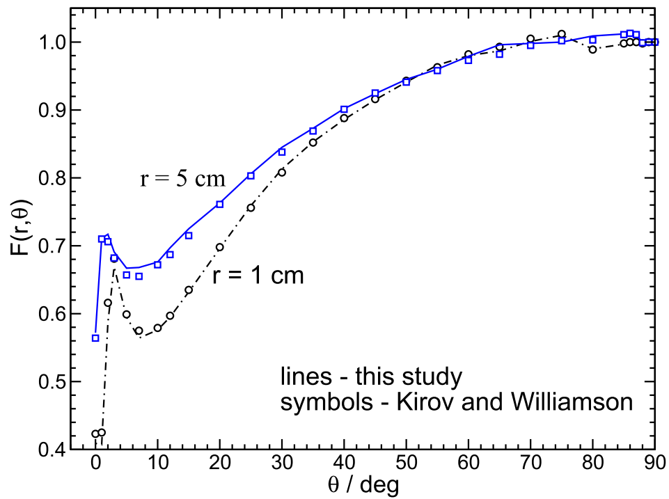
Figure 3.12: Comparisons of anisotropy data calculated for the STM1251 ^{125}\text{I} source with values calculated by Kirov and Williamson. 34 Voxel sizes are (0.1 \text{ mm})^3 at 1 cm and (0.5 \text{ mm})^3 at 5 cm. See figure 3.6 for values at 0.25 cm.
